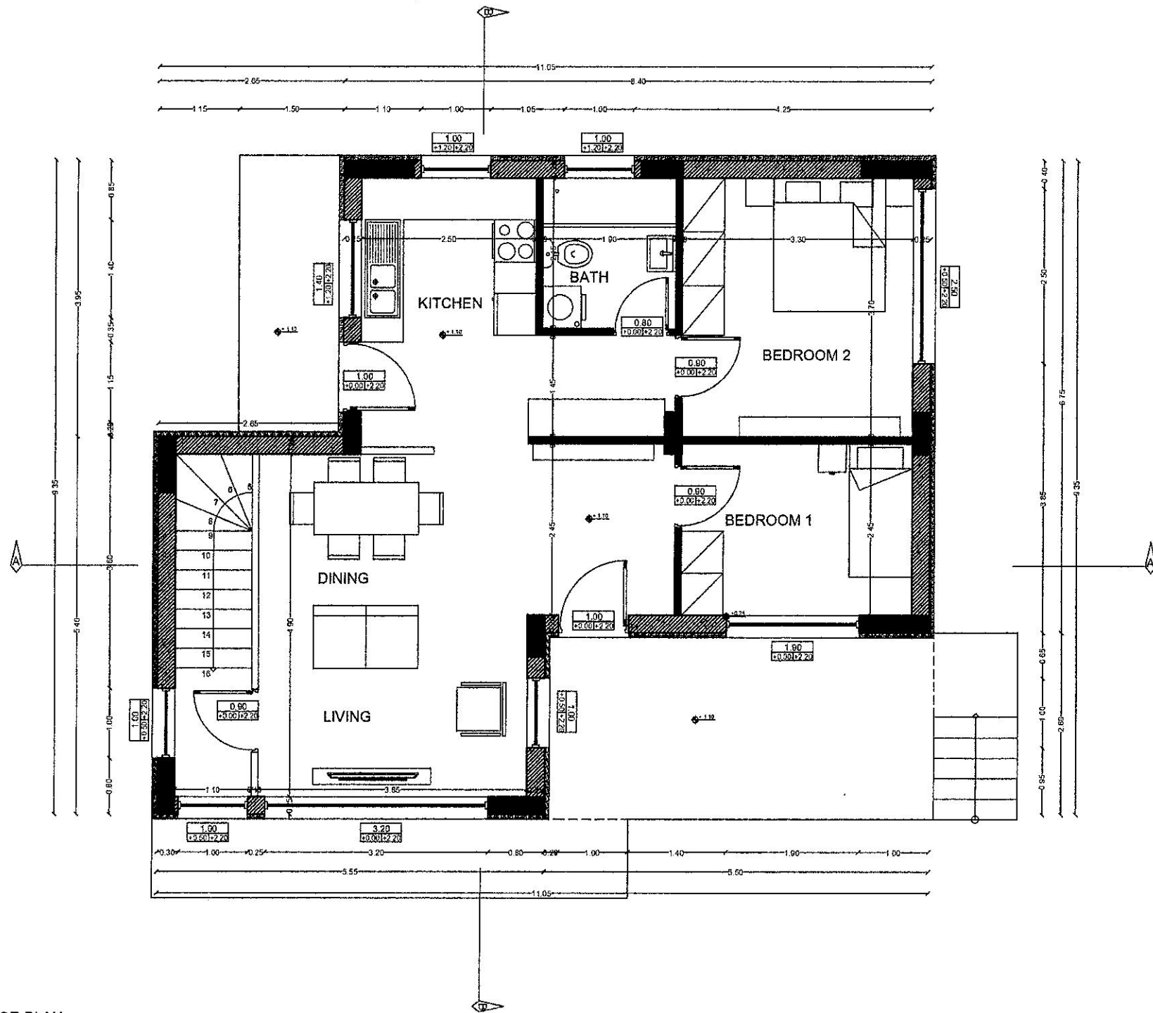
FLOOR PLAN
